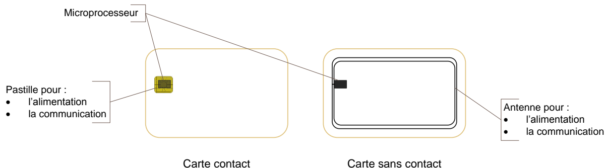
Figure 21 : technologie contact / sans-contact
